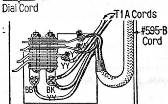
Connecting #595-B Cord and T1A Cords to Housing Contact Assembly
