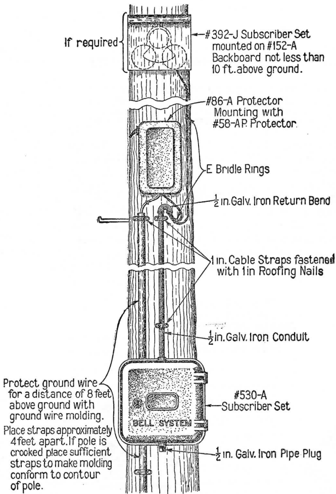
Figure 2. Pole Installation
