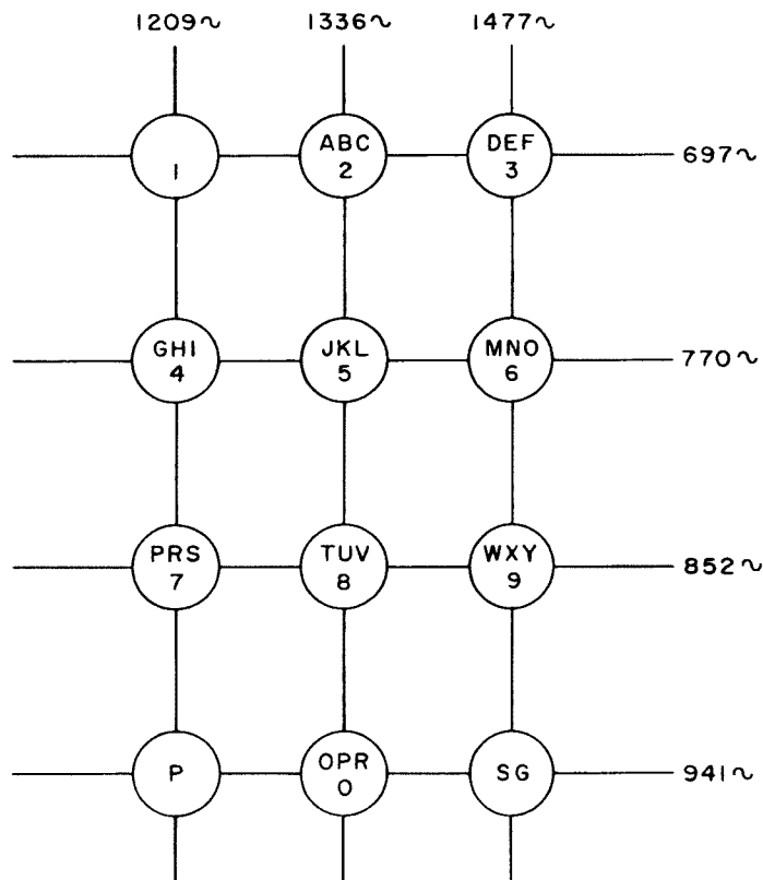
Fig. 3 - Dial Frequencies
