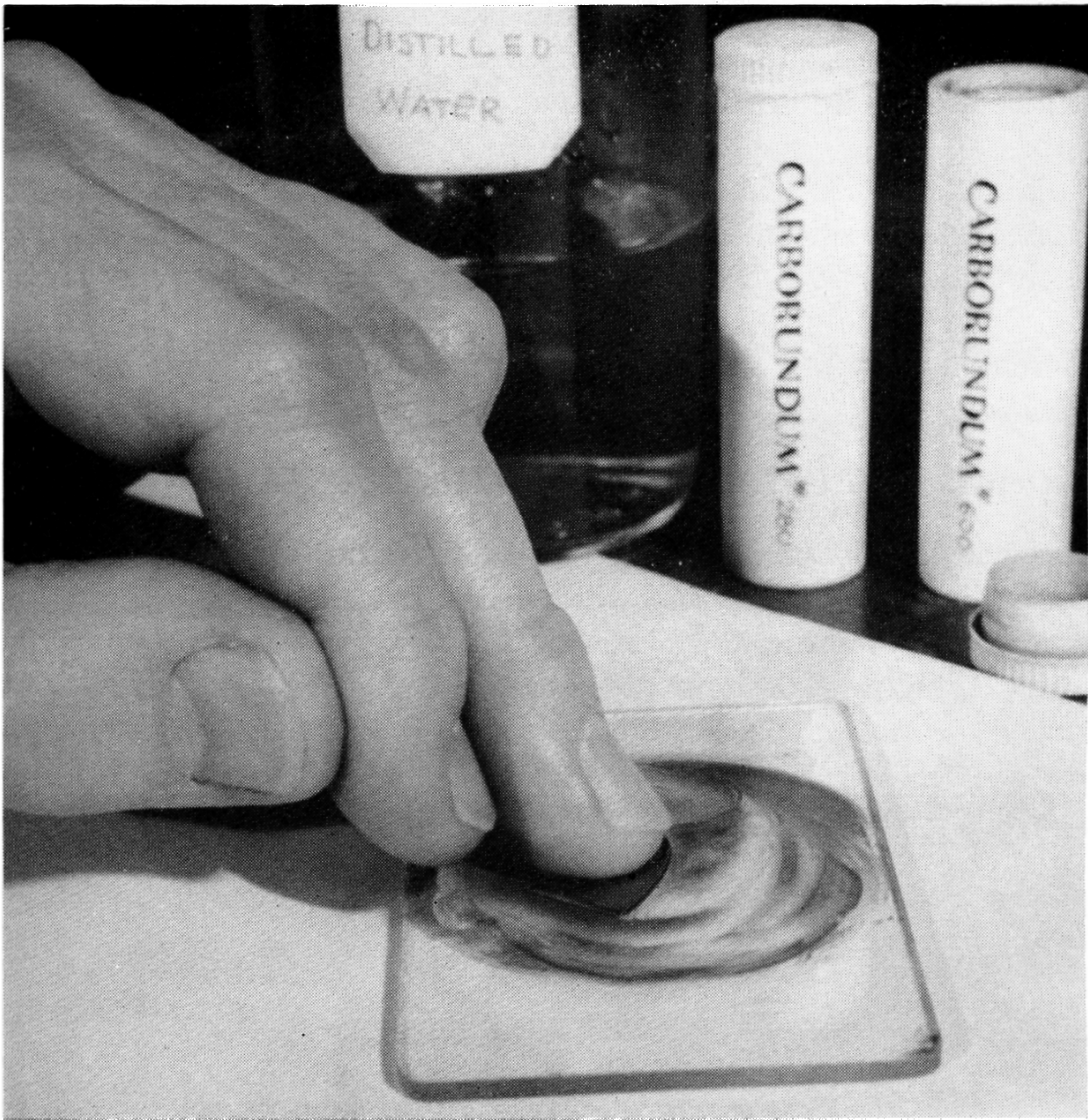
Figure 6-4. Grinding the silicon slab.
